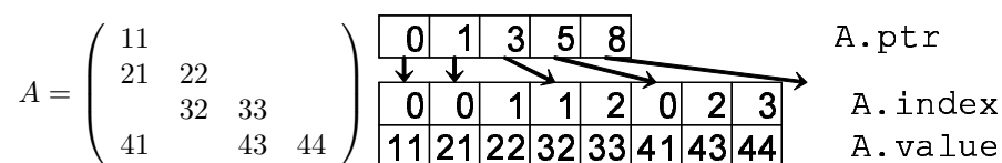
Figure 2: Data structure of CRS.
