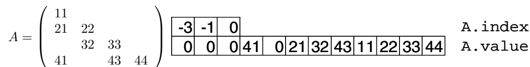
Figure 8: Data structure of DIA.
