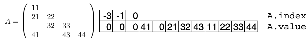
Figure 8: The data structure of the DIA format (for serial version).
