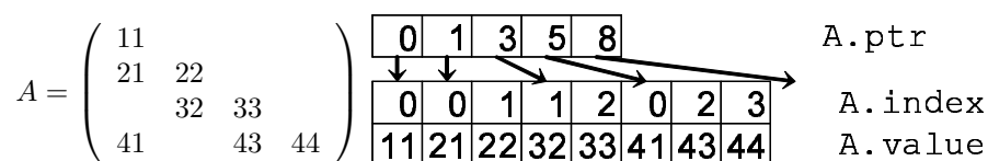
Figure 2: The data structure of the CRS format (for serial and OpenMP versions).
