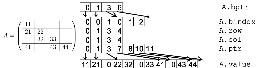
Figure 20: The data structure of the VBR format (for serial and OpenMP versions).
