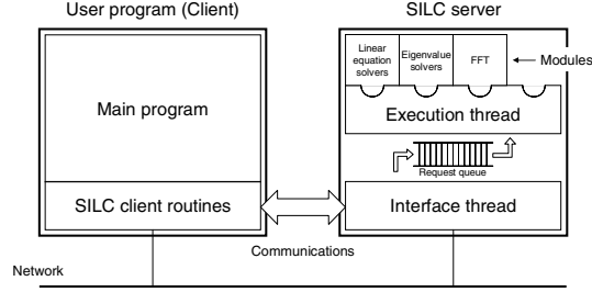
Fig. 1. Architectural overview of SILC.
